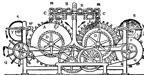
Fig. 39.—Section of Wordsworth's Flax-heckling Machine.
