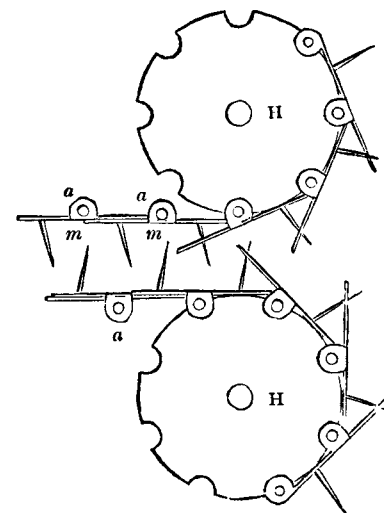
Fig. 25.—Machine for Wool Combing.
