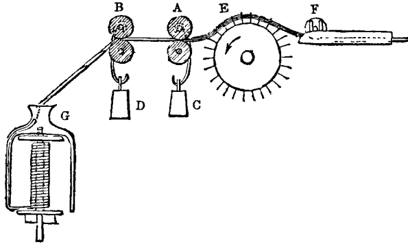
Fig. 27.—Worsted Roving.
