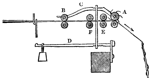
Fig. 29.—Worsted Throstle.
