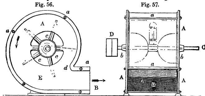
Fig. 56.—Side View of the Ventilating Fan. Fig. 57.—Front View of Ditto.
