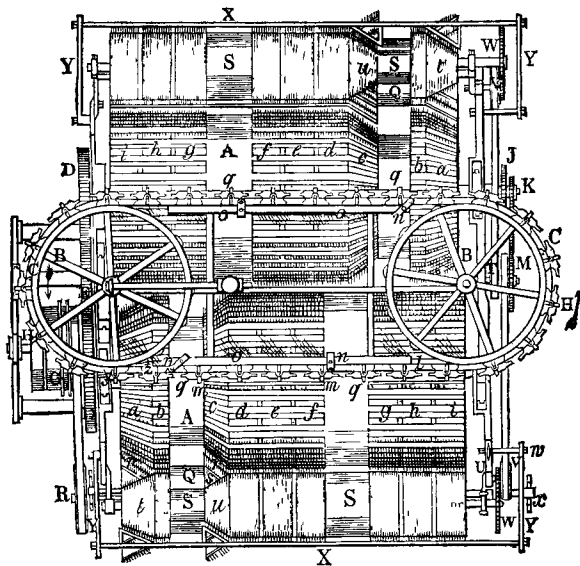
Fig. 38.—Plan of Wordsworth's Flax-heckling Machine.
