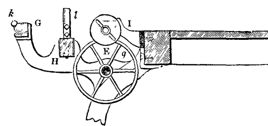
Fig. 48.—Bobbin Mechanism of the Silk Engine.
