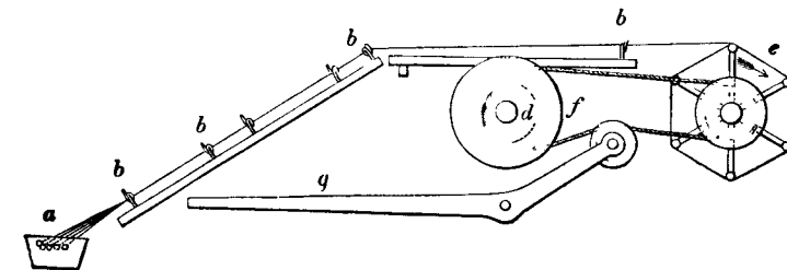
Fig. 46.—Cocoon Filature.—Section of Reel.
