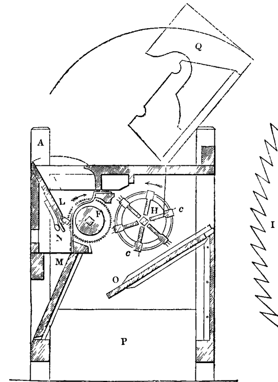
Fig. 17.—Whitney's Saw-gin.
