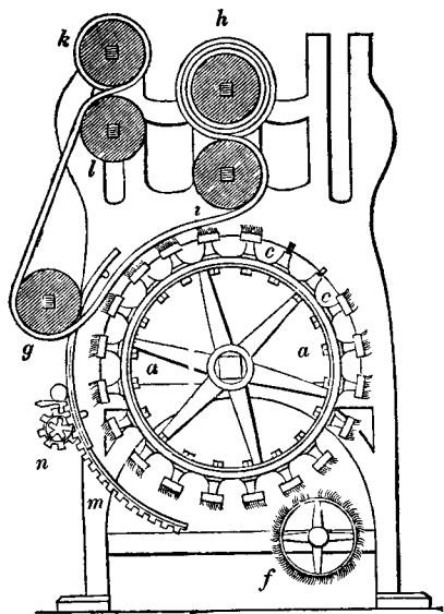
Fig. 35.—Atkinson's and Walker's Gig Mills united.
