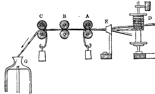
Fig. 28.—Worsted Spinning.
