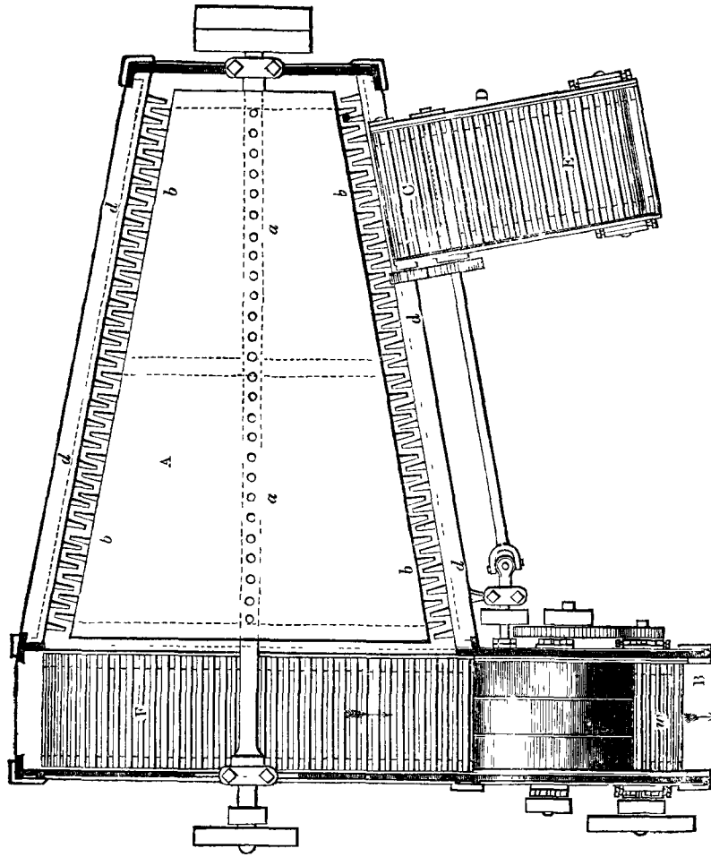
Fig. 30.—Lilly's Conical Willow.
