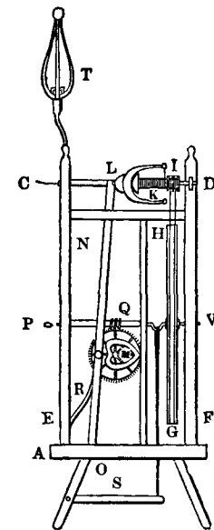
Fig. 44.—Self-acting Flax-wheel.
