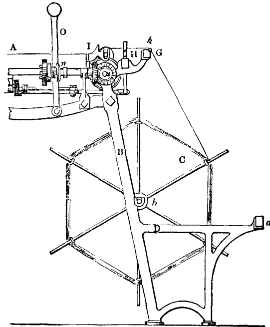
Fig. 47.—Silk-Engine, or Swift.
