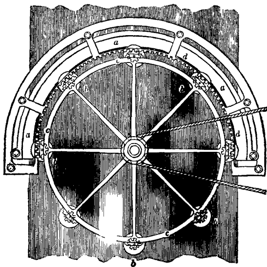
Fig 37.—Oldland's Cloth Shearing Machine.
