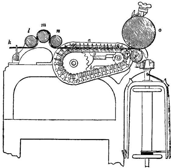
Fig. 40.—Wordsworth's Flax-roving Machine.
