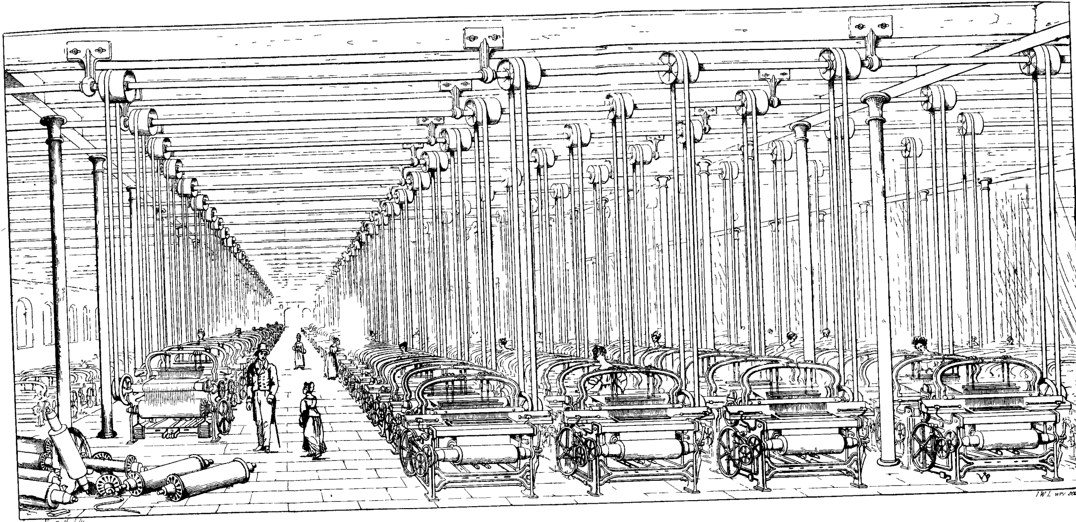
POWER LOOM FACTORY OF THOMAS ROBINSON ESQ R STOCKPORT.
