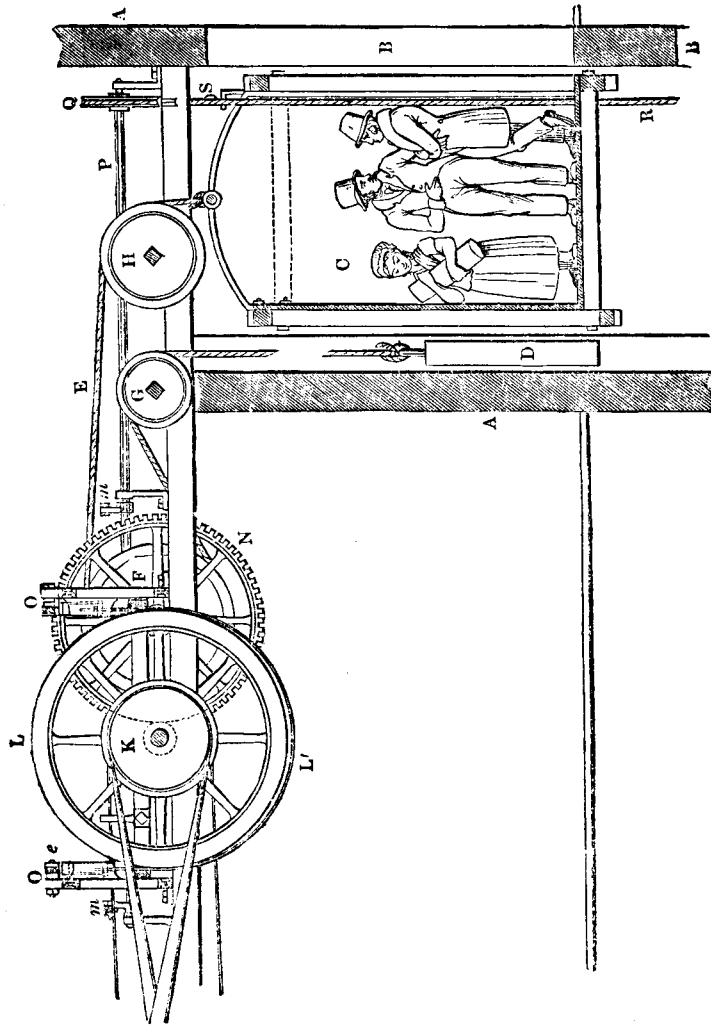
Fig. 1.—The Teagle.
