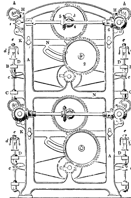
Fig 52 — End view of Fairbairn and Little's improved Silk Spinning-Mill.
